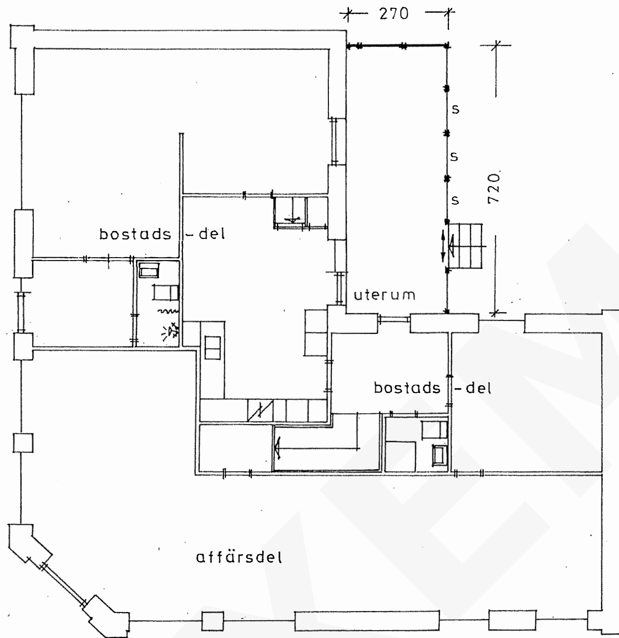
BOTTENPLAN
