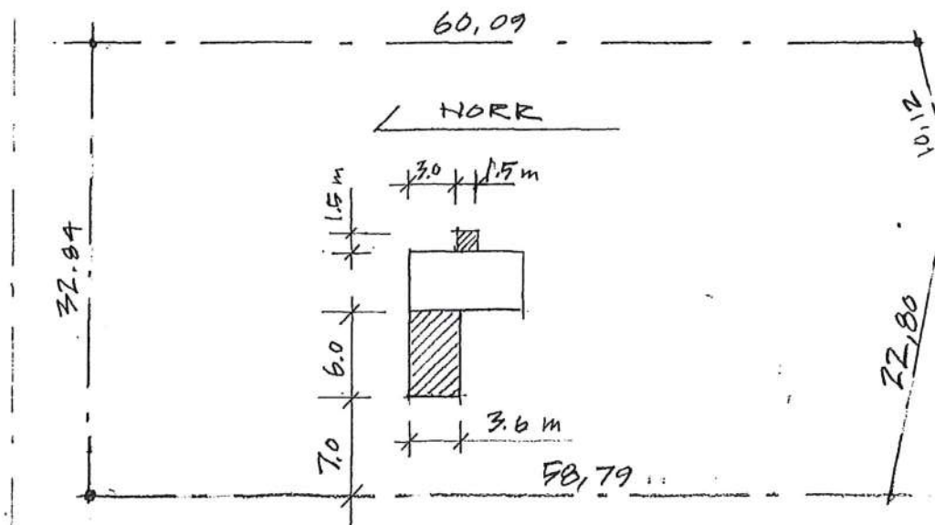
SITUATIONSPLAN skala 1:500
